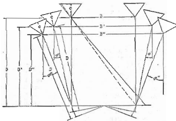
Figure 2 Convergent cases, equivalent normal case, and the overlap angle.
