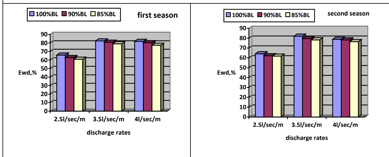
Fig.3 :Water distribution efficiency (Ewd, %) as affected by the combination of discharge rates and cut-off irrigation treatments during the two growing seasons
