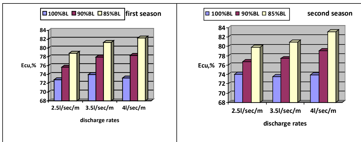
Fig.4 : Consumptive use efficiency (Ecu, %) as affected by the combination of discharge rates and cut-off irrigation treatments during the two growing seasons
