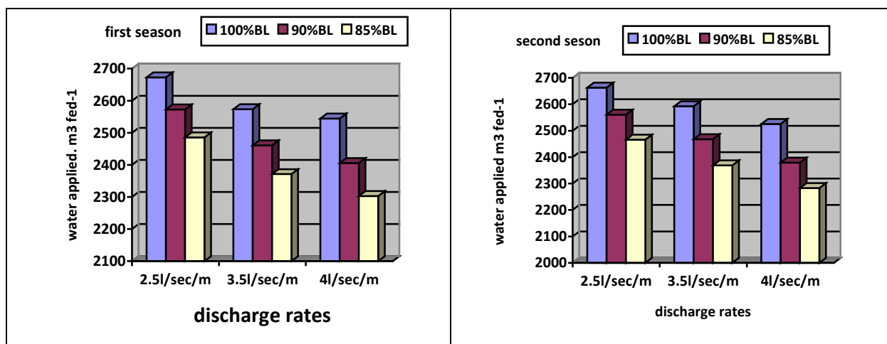
Fig. 1: Seasonal applied water (m 3 fed -1 ) for wheat crop as affected by discharge rates and cut-off irrigation treatments during the two growing seasons
