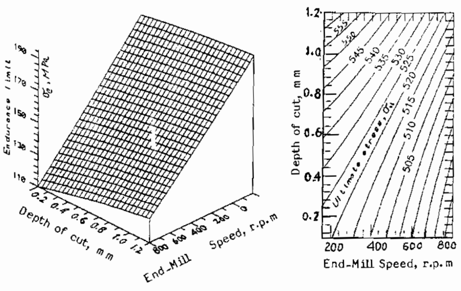
Fig. 6. Three-Dimensional and Contour Plots of the Endurance Limit versus Spindle Speed and Depth of Cut (Single-Side Milling)
