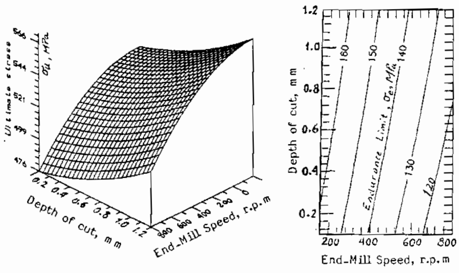
Fig. 5. Three-Dimensional and Contour Plots of the Ultimate Stress versus Spindle Speed and Depth of Cut (Single-side Milling)
