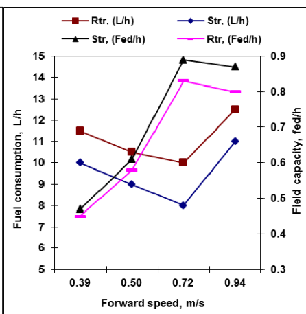
Fig (7): Effect of forward speed (V) on both field capacity (fed/h) and fuel consumption (L/h) in both two motion states
