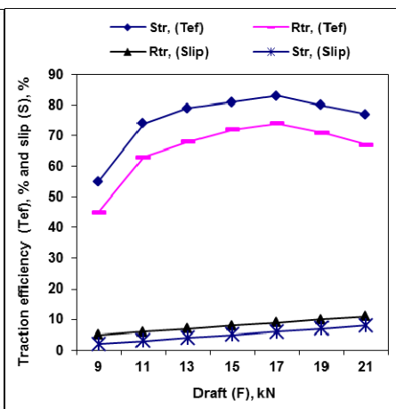
Fig (5): Effect of draft force (F) kN on both traction efficiency (Tef) % and slip (S) % in straight line
