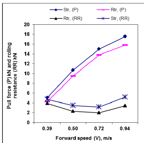
Fig (6): Effect of forward speed (V) on both pull force (P) kN and rolling resistance force (RR) kN in straight line
