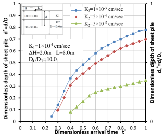
Fig. 7. Relationship between dimensionless depth of sheet pile and dimensionless arrival time for different permeability for the lower layer.
