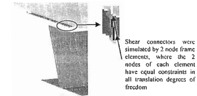
Figure (6). Shear connectors
