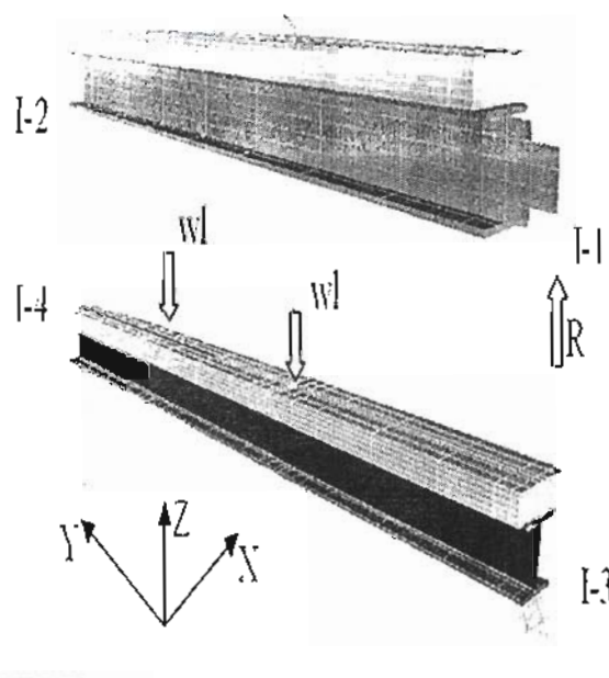
Figure (2), Finite element model case 1
