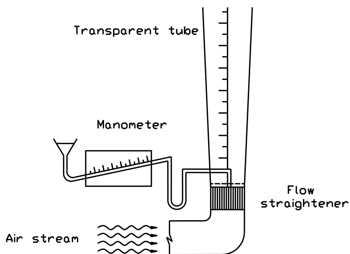
Fig. (1) The mechanism that was used for testing peanut aerodynamic properties.
