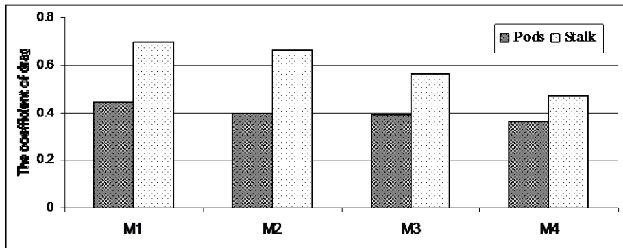
Fig. (5): Relation between different levels of moisture content and the coefficient of drag for pods and stalk pieces.
