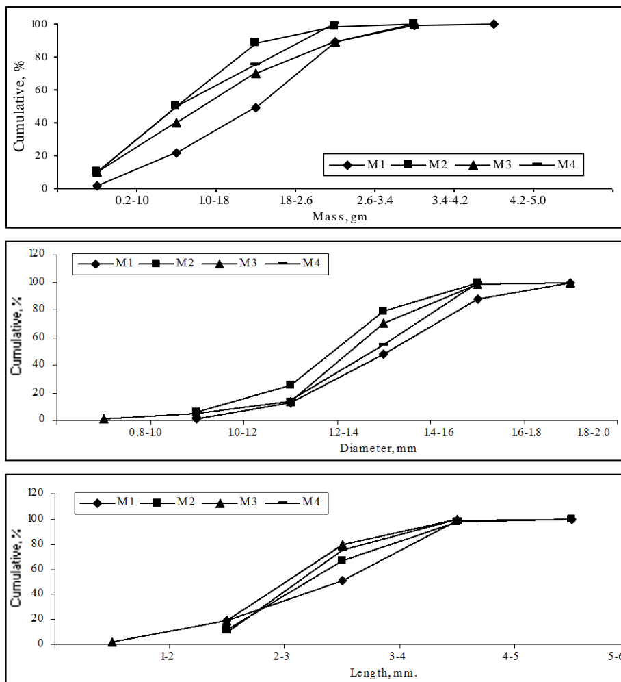
Fig. (3): Cumulative curves for mass, diameter and length of peanut pods, at four levels of moisture content.
