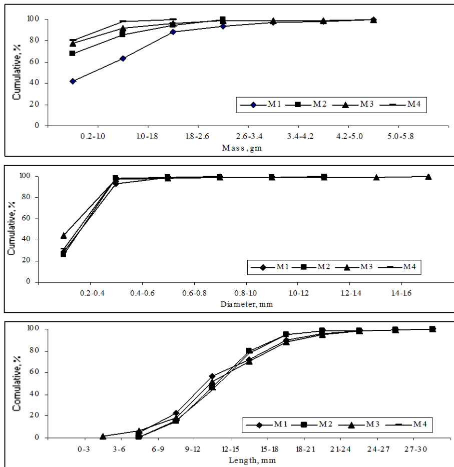
Fig. (2) Cumulative curves for mass, diameter and length of peanut stalk pieces, at four levels of moisture content.
