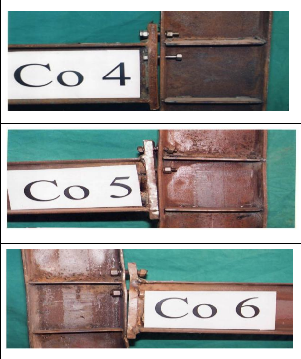
Fig. (26): Modes of Failure for the tested connections (Co.4, Co.5 & Co.6) in the group II
