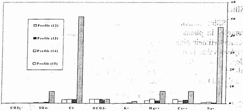
Fig.(5): Averages of cations and anions variability histogram (in meq/L) of Wadi Nasseib.
