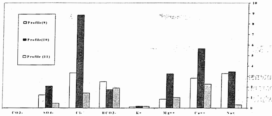
Fig.(5): Averages of cations and anions variability histogram (in meq/L) of Wadi Nasseib.
