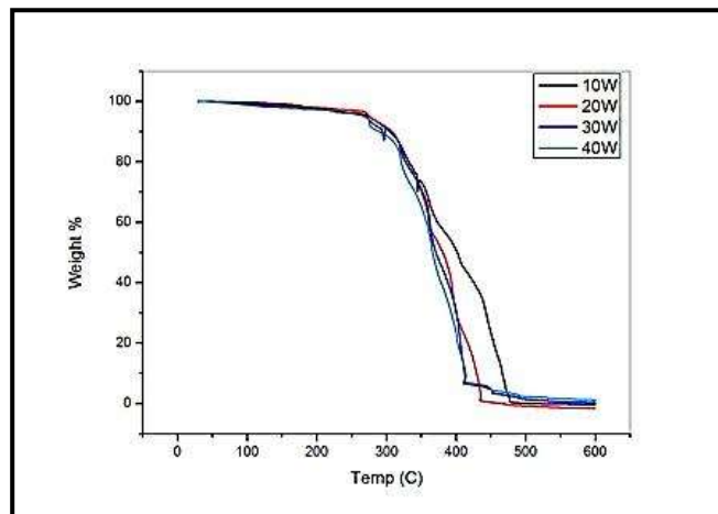
Fig. 3.6. TGA curve of WPCs
