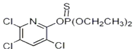
Fig.2: Chlorpyrifos
