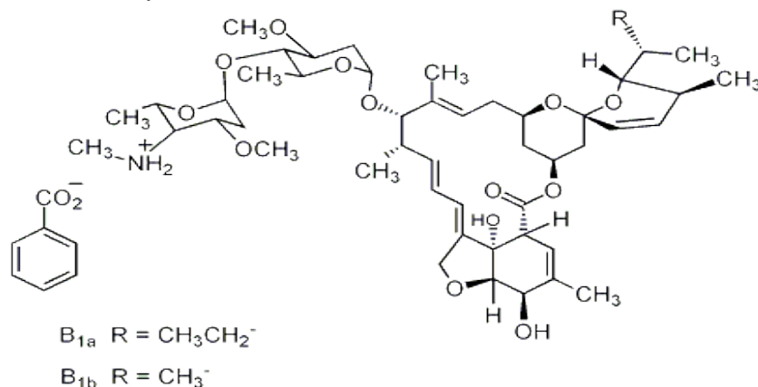
Fig. 1: Emamectin benzoate
