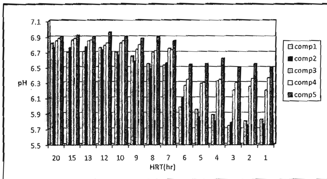
Figure 6 pH of the GRABBR at different HRT
