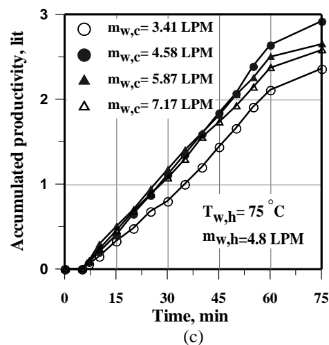
Fig. 5. The variation of accumulated productivity with time at the different cooling water mass flow rate and \dot{m}_{w,h} = 4.8 LPM.
