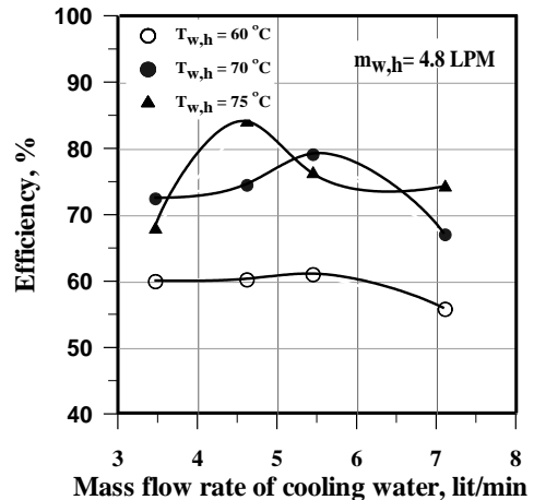
Fig.8 The variation of efficiency with cooling water mass flow rate at different inlet heating brackish water temperatures.
