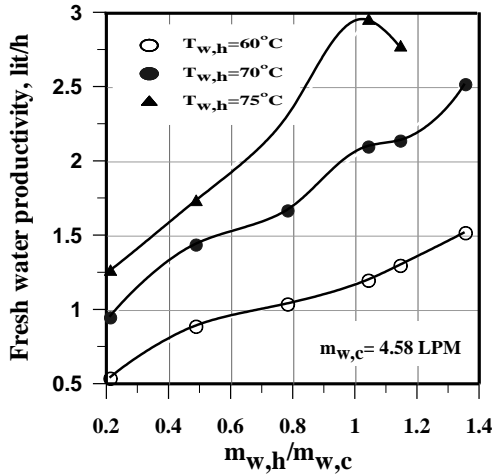
Fig. 9 The variation of fresh water productivity with the ratio (m_{w,h}/m_{w,c}) at different inlet heating brackish water temperatures..
