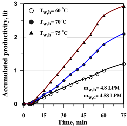
Fig.6 Variation of accumulated productivity with time at different inlet heating brackish water temperatures.
