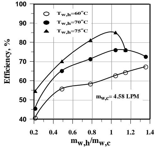
Fig.10 The variation of efficiency with the ratio (m_{w,h}/m_{w,c}) at different inlet heating brackish water temperatures.
