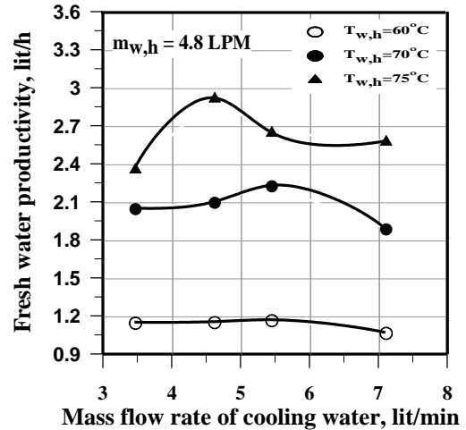
Fig.7 The variation of fresh water productivity with the cooling water mass flow rate at different inlet heating brackish water temperatures.
